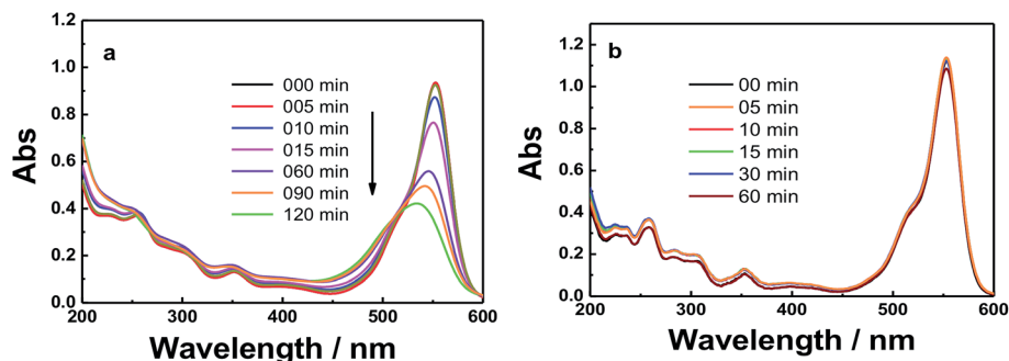
Fig. 8 Absorbance spectra of RhB dye in the presence of: (a) GO and (b) GO-Fe 3 O 4 @ZrO 2 at the indicated time intervals under irradiation.
